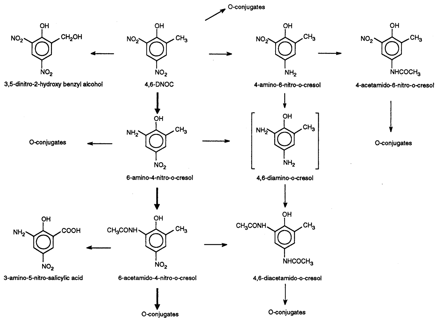
FIGURE 2-3. Metabolic Pathways for 4,6-Dinitro-o-cresol*
